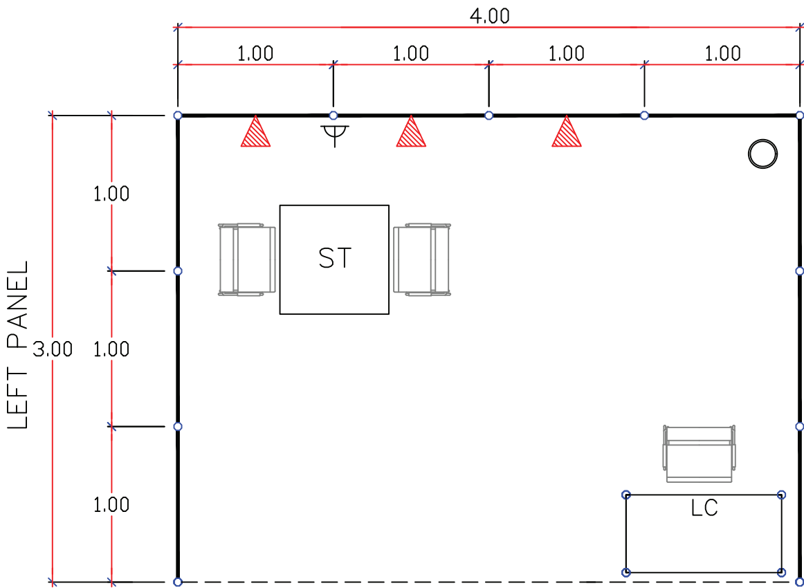
FRONT SIDE LAY-OUT
